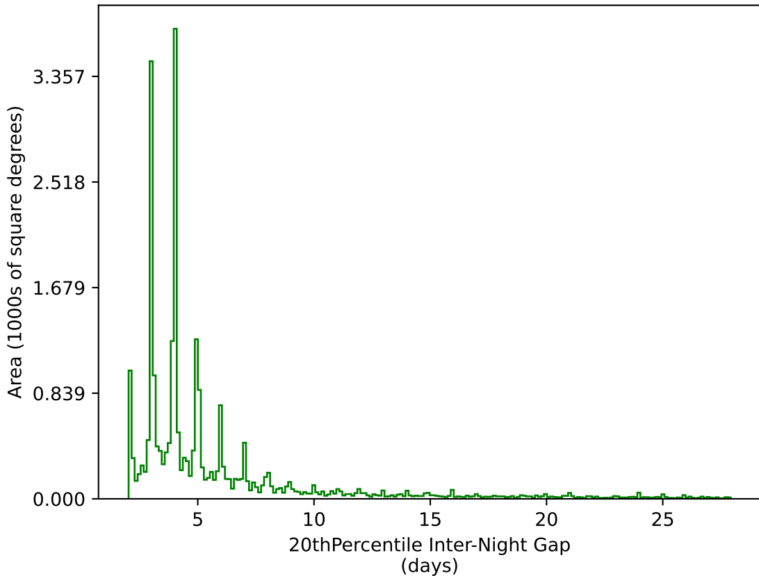
weather_cloudso6v3.4_10yrs All sky g band: 20thPercentile Inter-Night Gap
