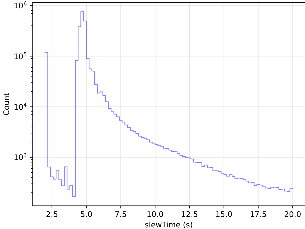
weather_cloudso6v3.4_10yrs All visits: Zoom Slew Time Histogram
