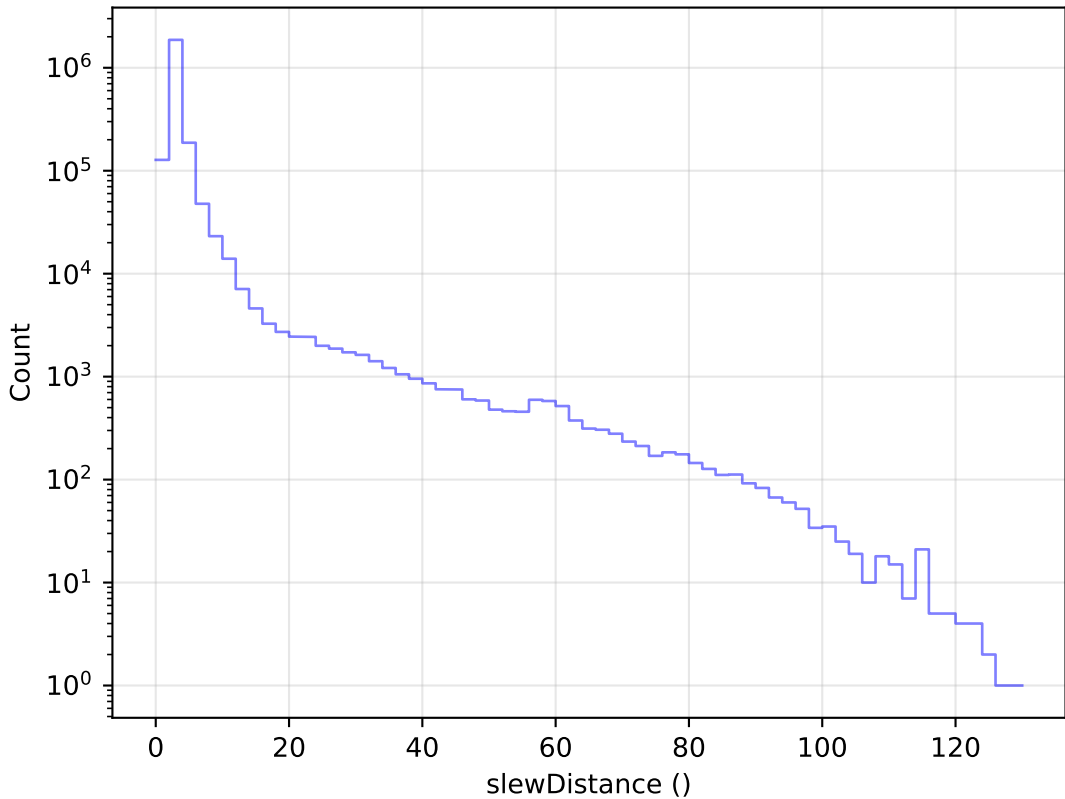
weather_cloudso6v3.4_10yrs All visits: Slew Distance Histogram
