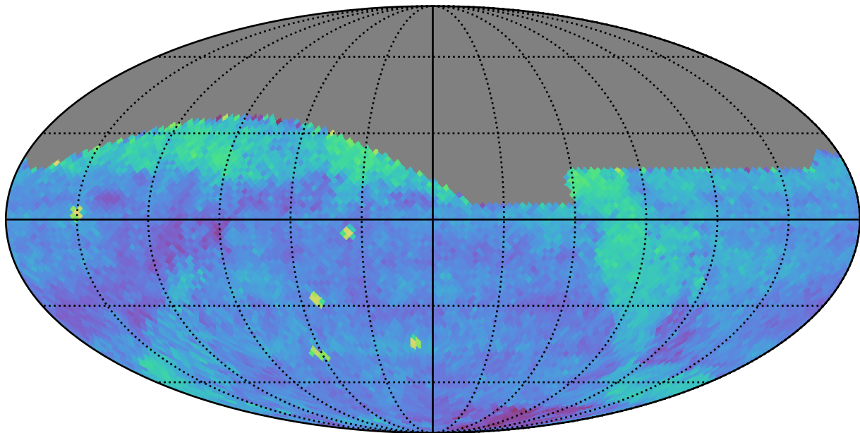
weather_cloudso6v3.4_10yrs (g or r or i): PairFraction
