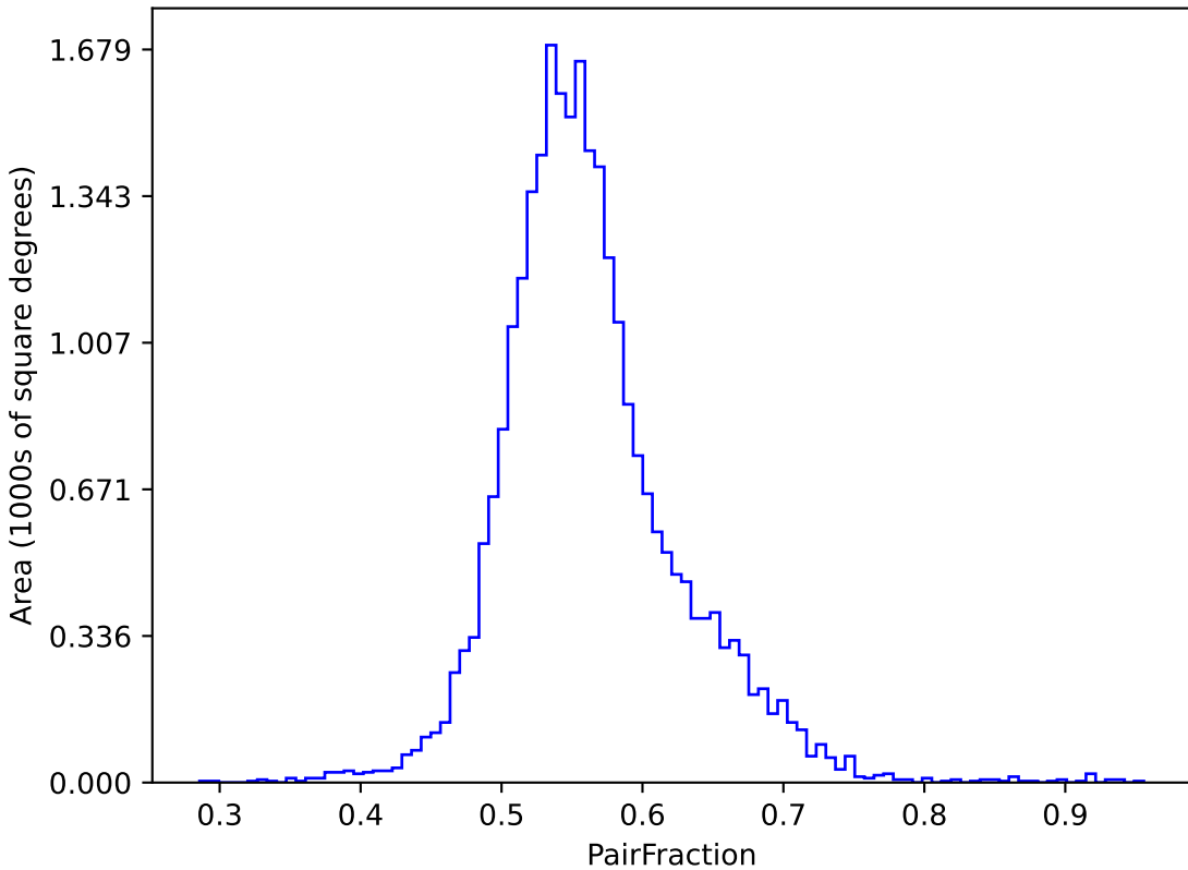
weather_cloudso6v3.4_10yrs (g or r or i): PairFraction
