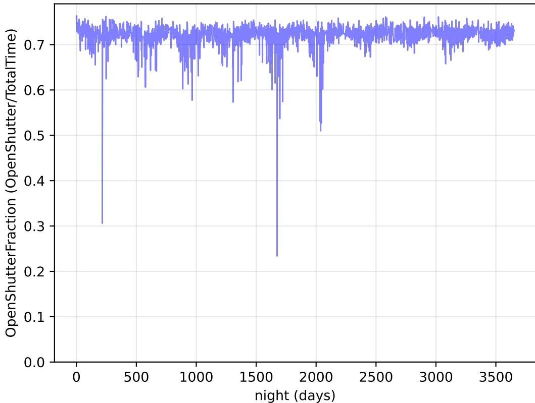
weather_cloudso6v3.4_10yrs : OpenShutterFraction
