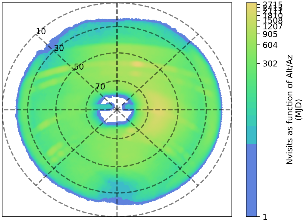
weather_cloudso6v3.4_10yrs z: Nvisits as function of Alt/Az
