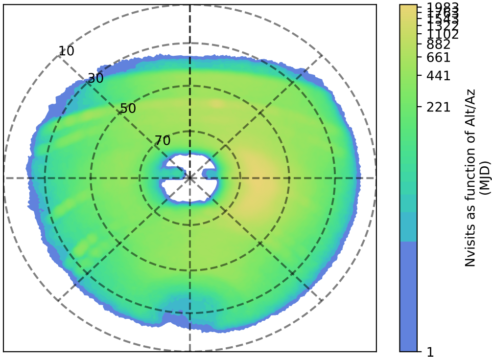
weather_cloudso6v3.4_10yrs y: Nvisits as function of Alt/Az
