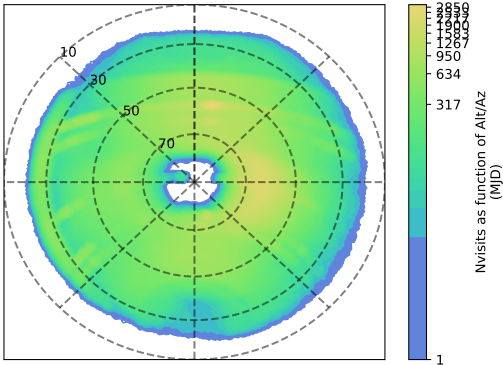
weather_cloudso6v3.4_10yrs r: Nvisits as function of Alt/Az
