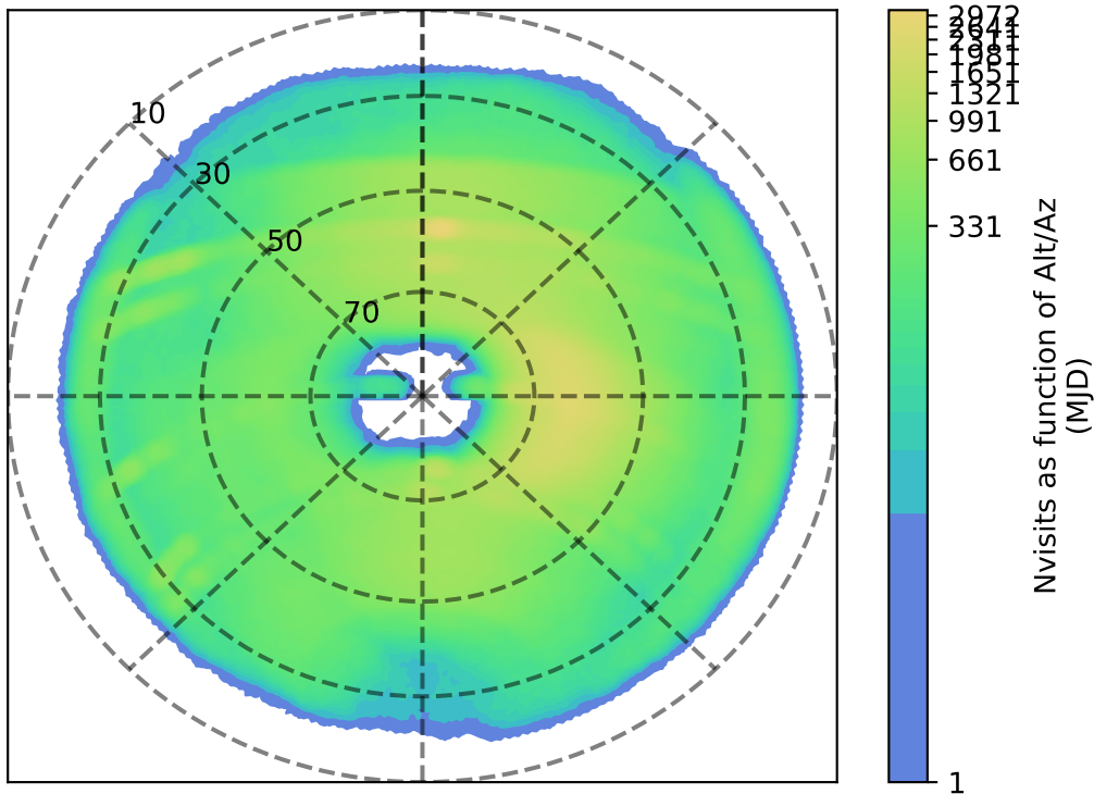
weather_cloudso6v3.4_10yrs i: Nvisits as function of Alt/Az
