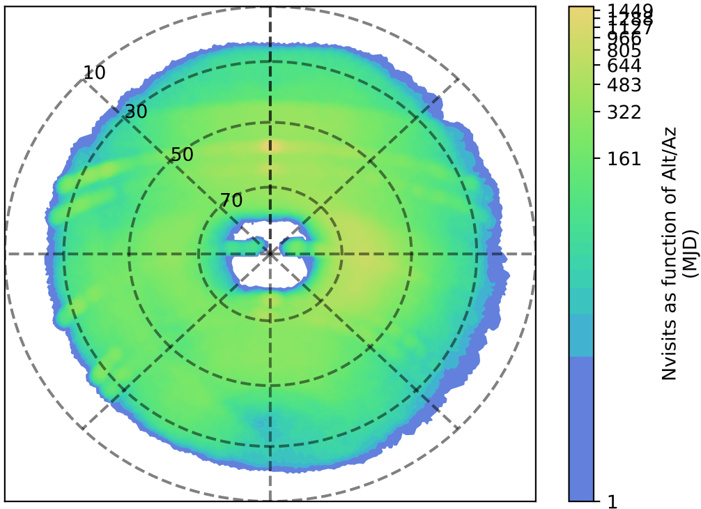
weather_cloudso6v3.4_10yrs g: Nvisits as function of Alt/Az
