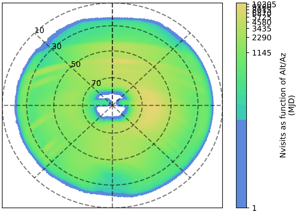
weather_cloudso6v3.4_10yrs : Nvisits as function of Alt/Az
