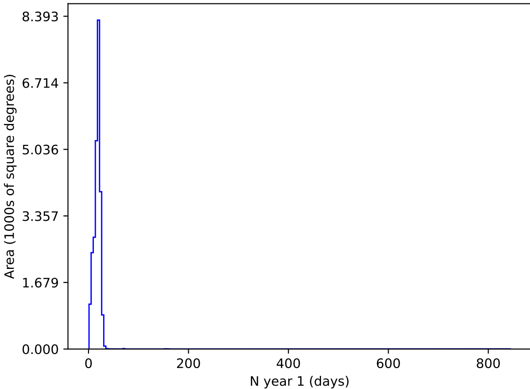
weather_cloudso6v3.4_10yrs y and night < 365: N year 1
