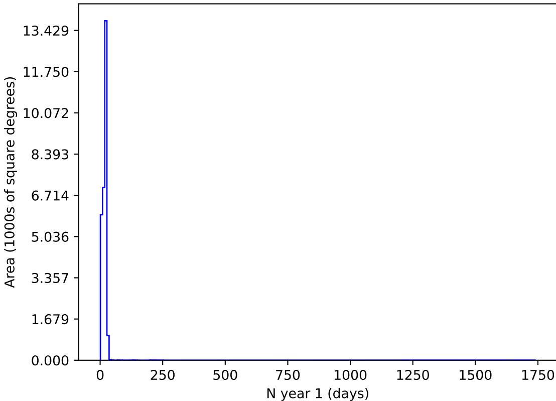
weather_cloudso6v3.4_10yrs i and night < 365: N year 1
