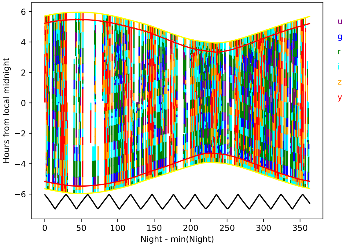
weather_cloudso6v3.4_10yrs year 9-10: Hourglass
