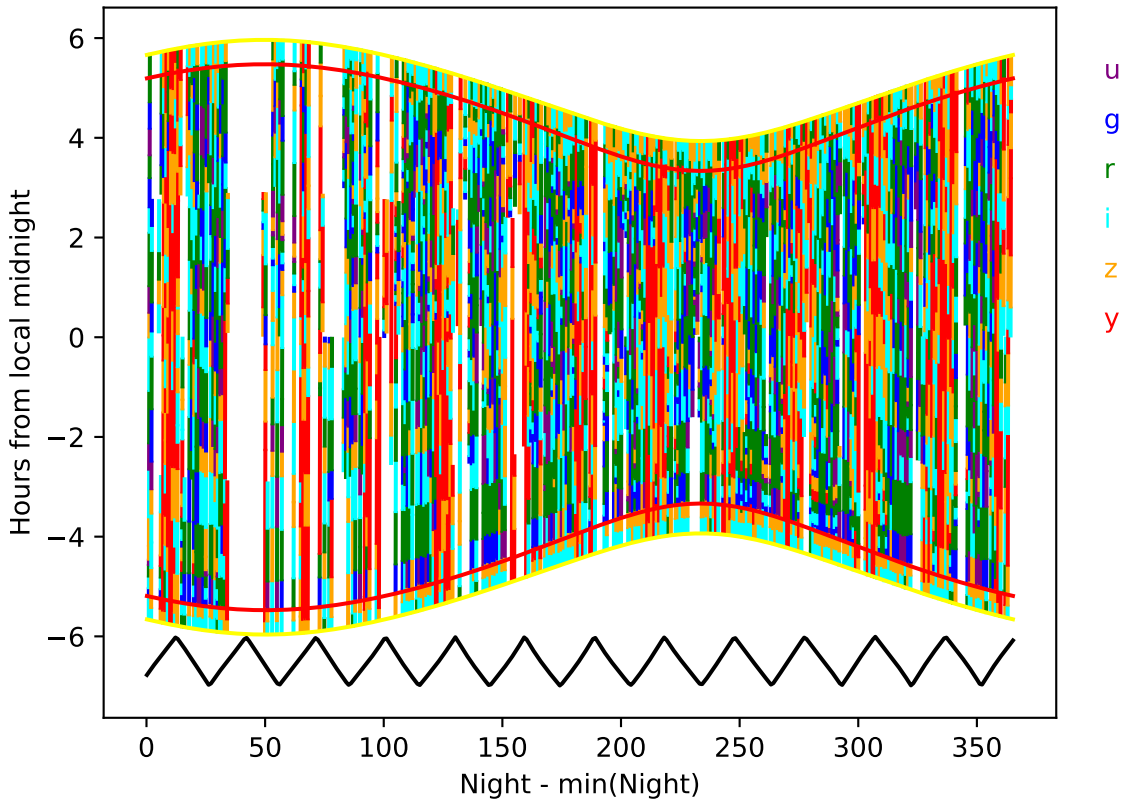
weather_cloudso6v3.4_10yrs year 8-9: Hourglass
