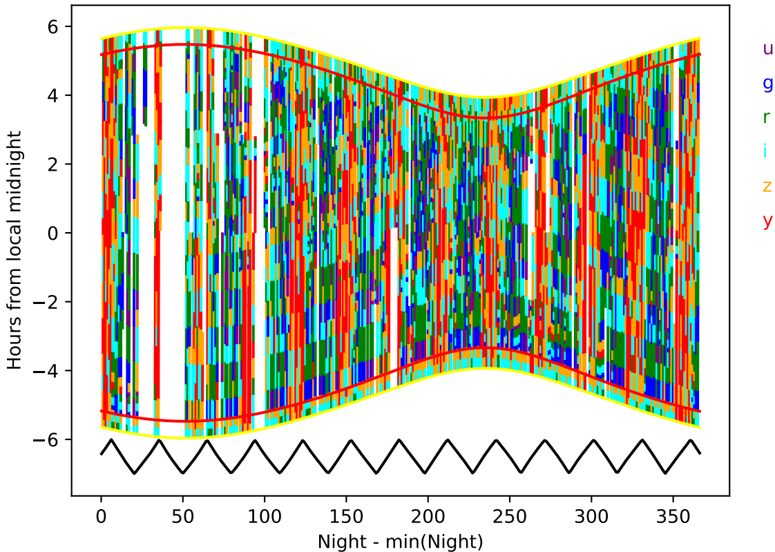
weather_cloudso6v3.4_10yrs year 6-7: Hourglass
