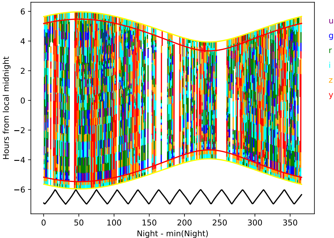
weather_cloudso6v3.4_10yrs year 5-6: Hourglass
