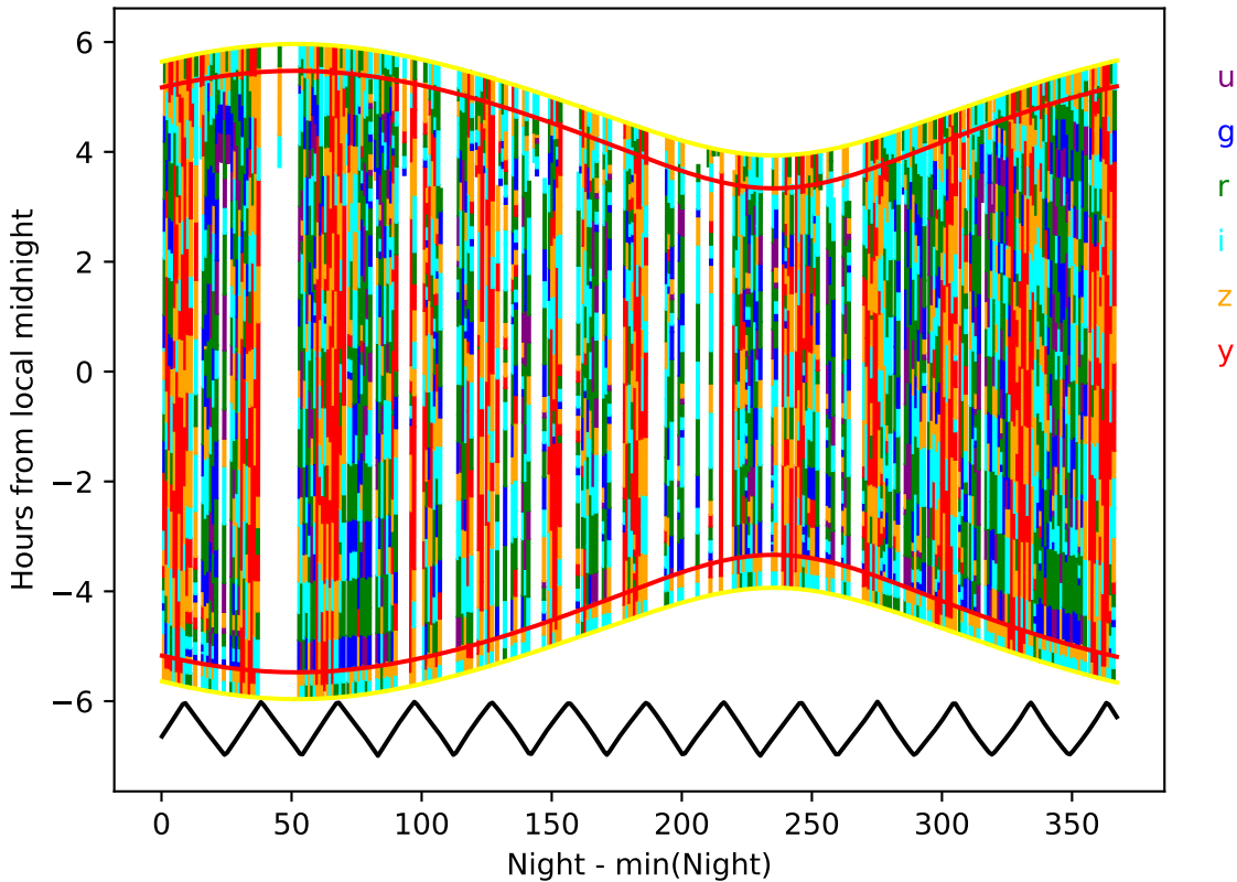
weather_cloudso6v3.4_10yrs year 3-4: Hourglass
