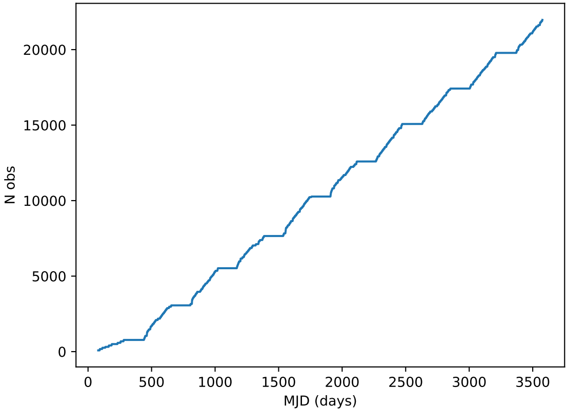
weather_cloudso6v3.4_10yrs note like DD:XMM_LSS%: Cumulative
