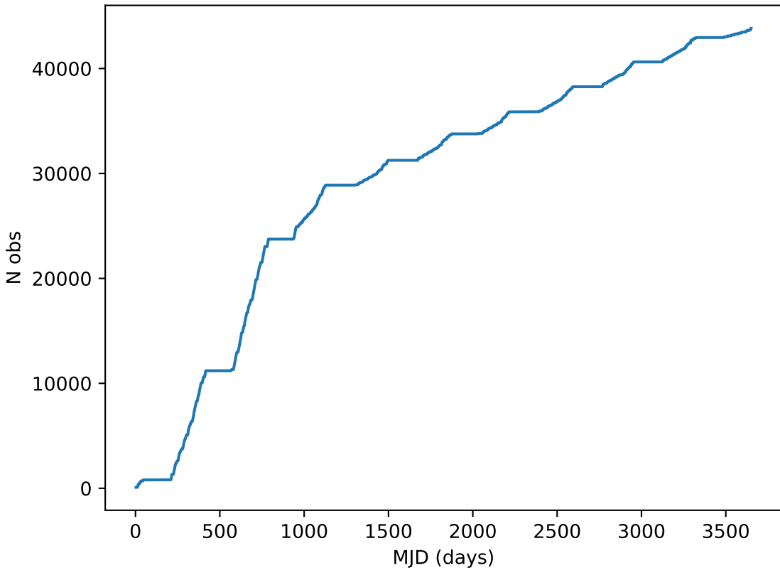
weather_cloudso6v3.4_10yrs note like DD: COSMOS%: Cumulative
