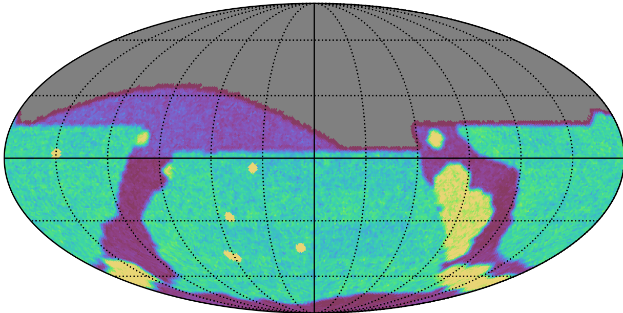
weather_cloudso6v3.4_10yrs g: Count observationStartMJD
