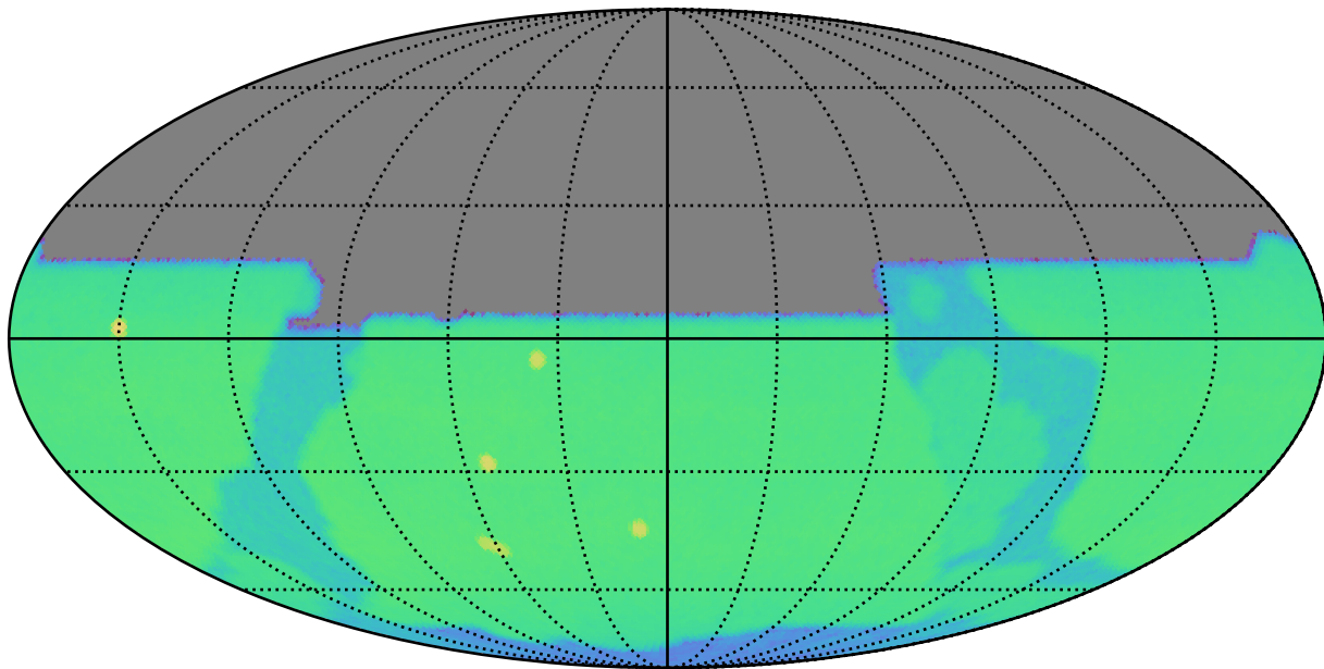
weather_cloudso6v3.4_10yrs y: CoaddM5
