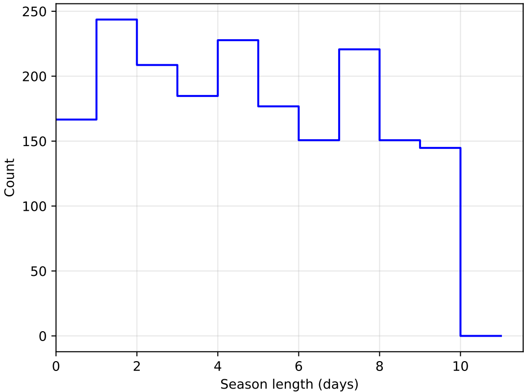
weather_cloudso6v3.4_10yrs DD:WFD all bands: SeasonLength
