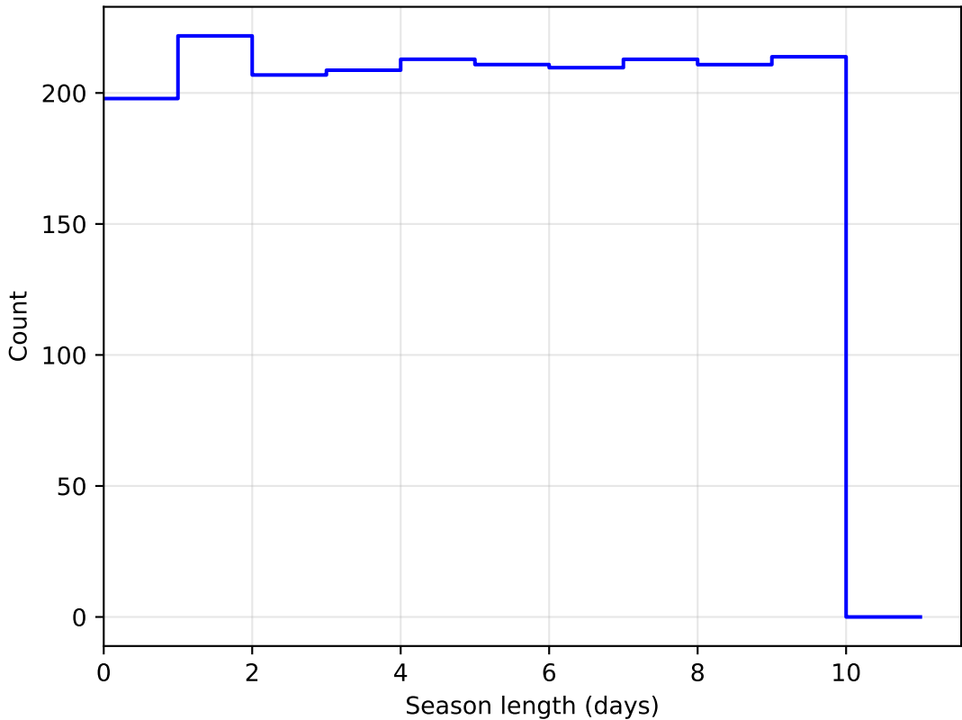
weather_cloudso6v3.4_10yrs DD:ELAISS1 all bands: SeasonLength
