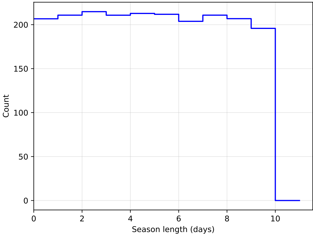
weather_cloudso6v3.4_10yrs DD:EDFS all bands: SeasonLength
