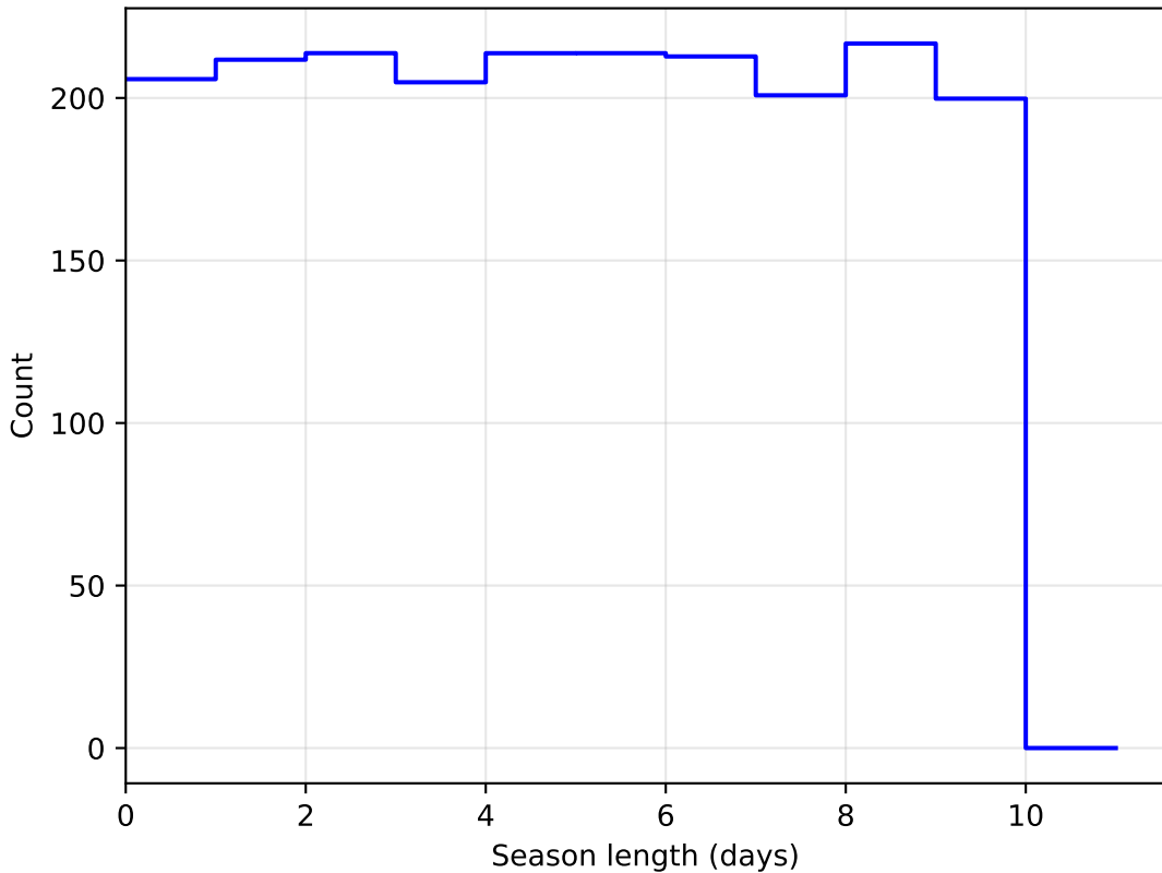
weather_cloudso6v3.4_10yrs DD:ECDFS all bands: SeasonLength
