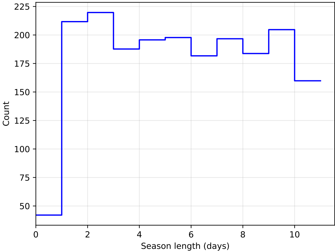
weather_cloudso6v3.4_10yrs DD: COSMOS all bands: SeasonLength
