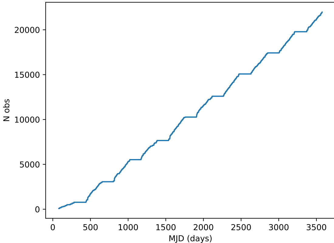
weather_cloudso6v3.4_10yrs all bands: DD:XMM_LSS Cumulative NVisits
