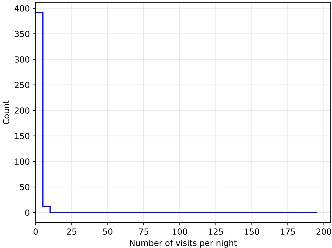
weather_cloudso6v3.4_10yrs all bands: DD:WFD NVisitsPerNight
