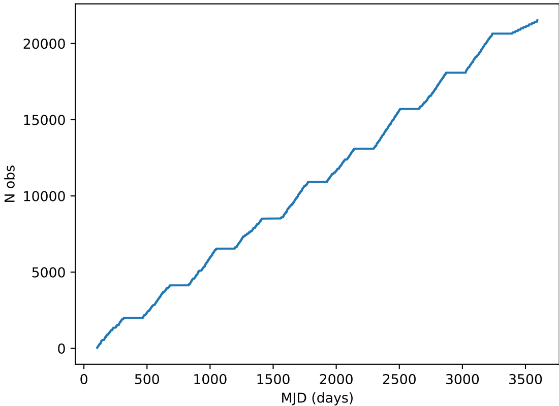
weather_cloudso6v3.4_10yrs all bands: DD:EDFS Cumulative NVisits
