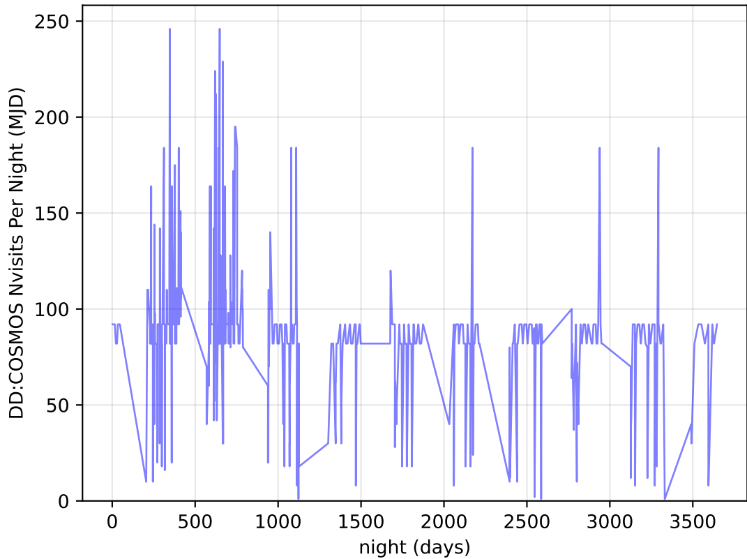
weather_cloudso6v3.4_10yrs all bands: DD: COSMOS Nvisits Per Night
