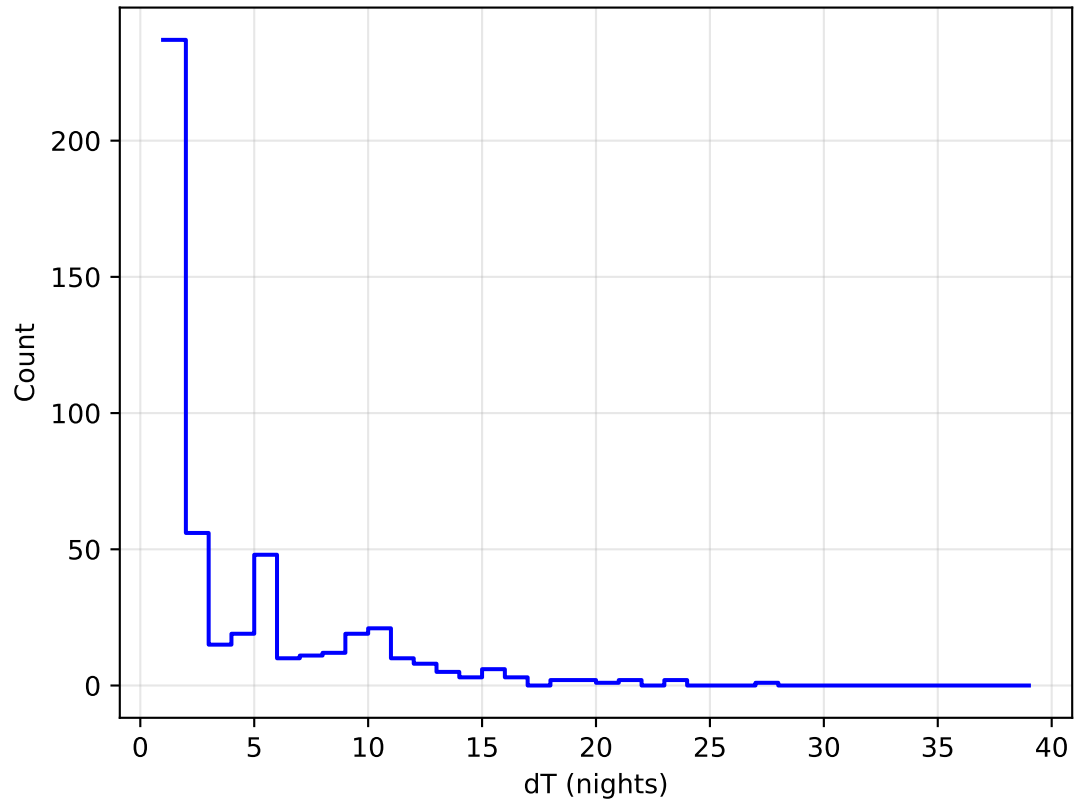
weather_cloudso6v3.4_10yrs all bands: DD: COSMOS Delta Nights Histogram
