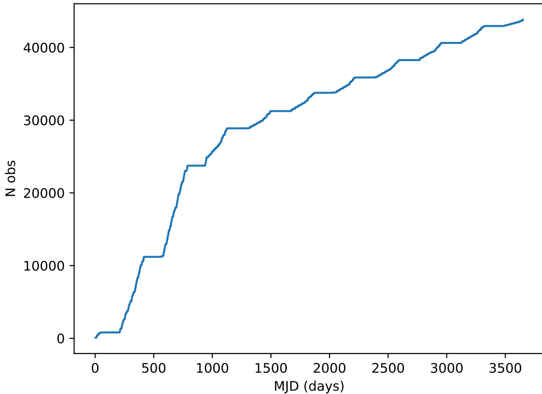
weather_cloudso6v3.4_10yrs all bands: DD:COSMOS Cumulative NVisits
