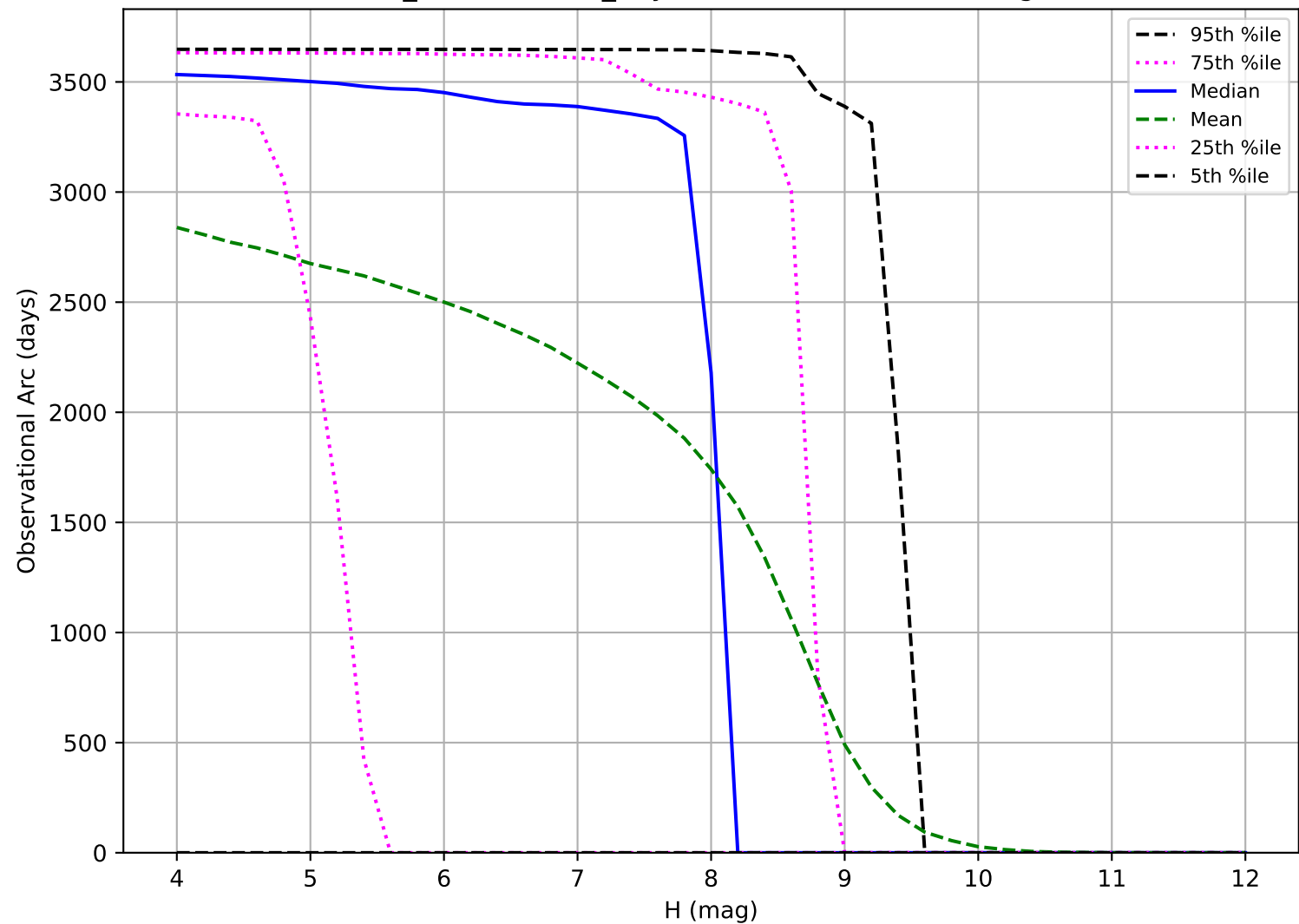
weather_cloudso4v3.4_10yrs: Observational Arc Length TNO
