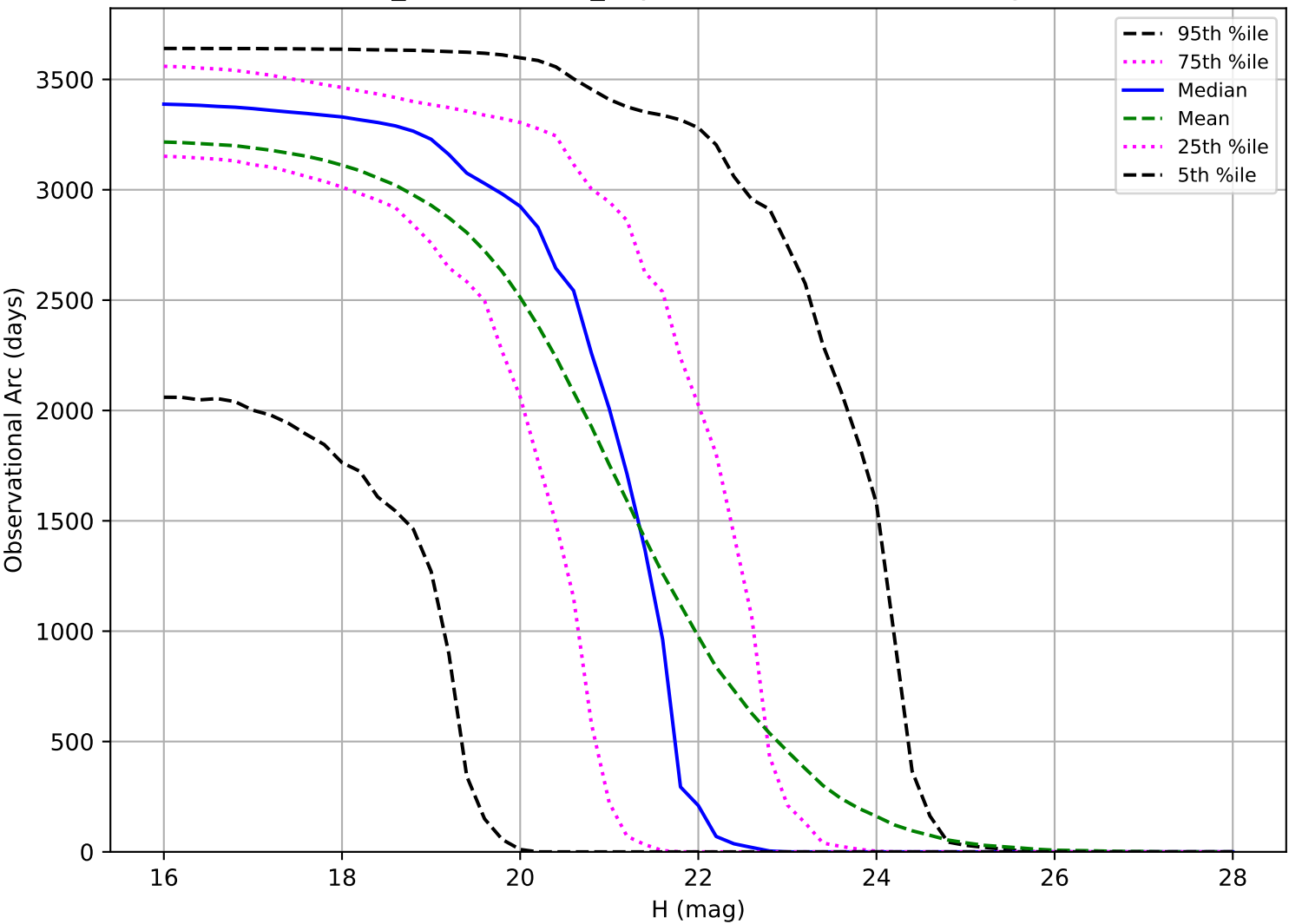
weather_cloudso4v3.4_10yrs: Observational Arc Length PHA
