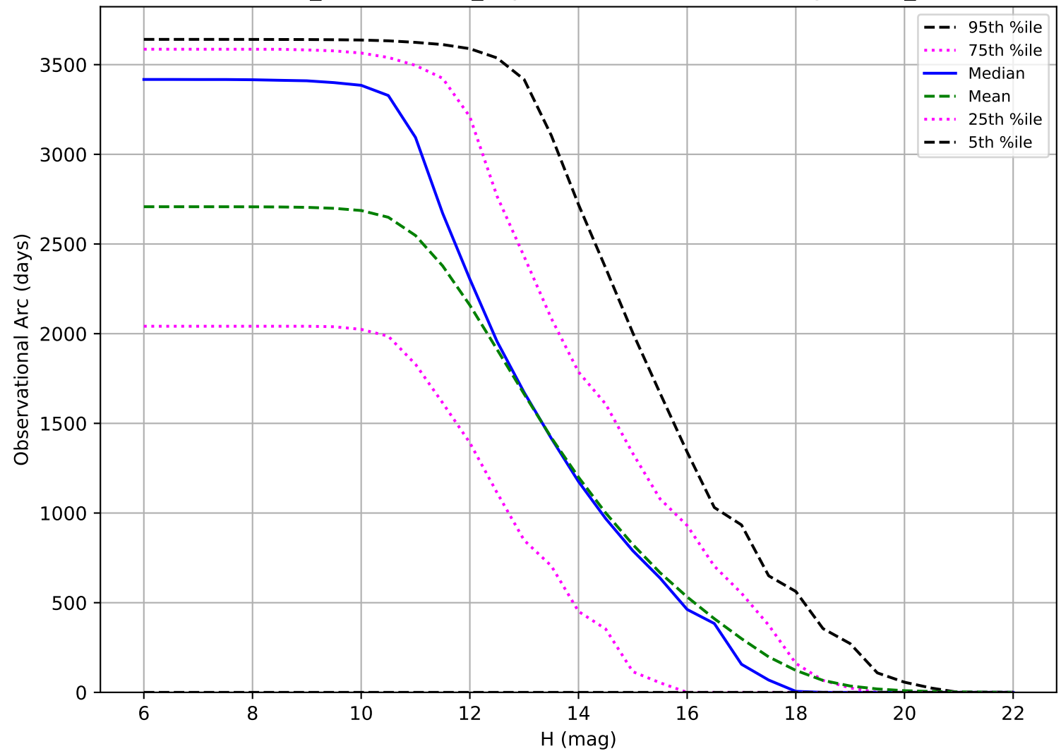
weather_cloudso4v3.4_10yrs: Observational Arc Length OCC_r5
