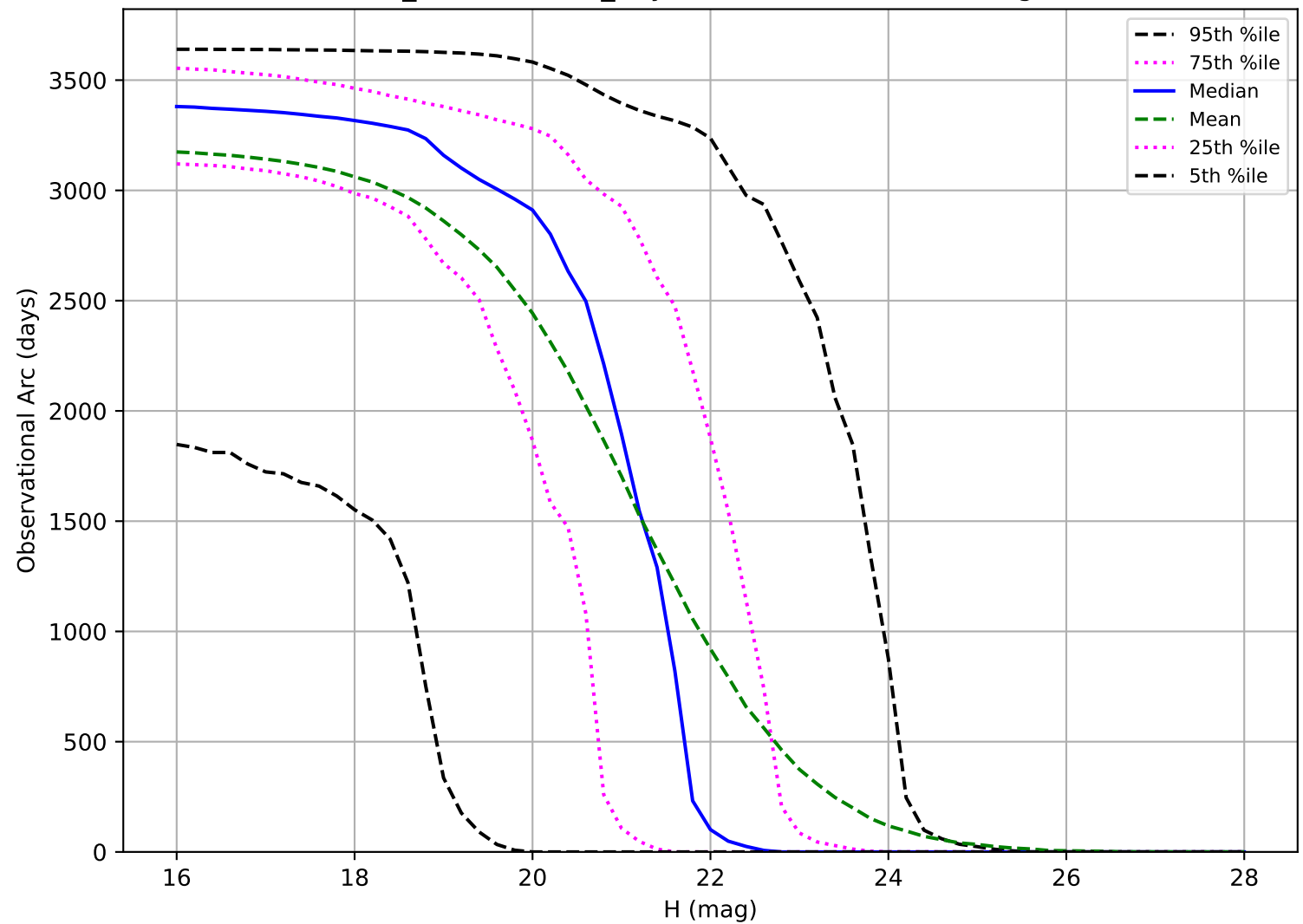
weather_cloudso4v3.4_10yrs: Observational Arc Length NEO
