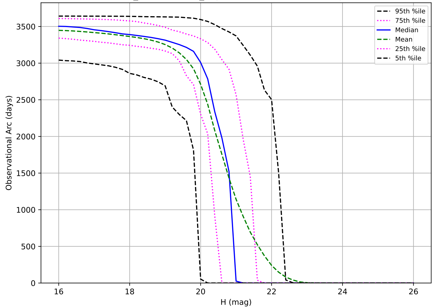
weather_cloudso4v3.4_10yrs: Observational Arc Length MBA
