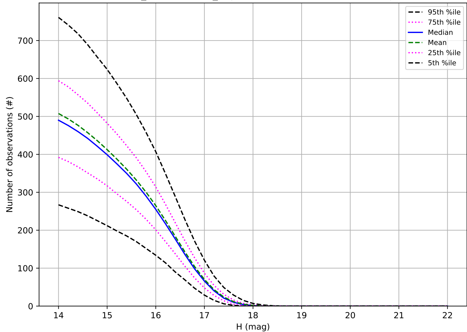
weather_cloudso4v3.4_10yrs: Number of observations Trojan
