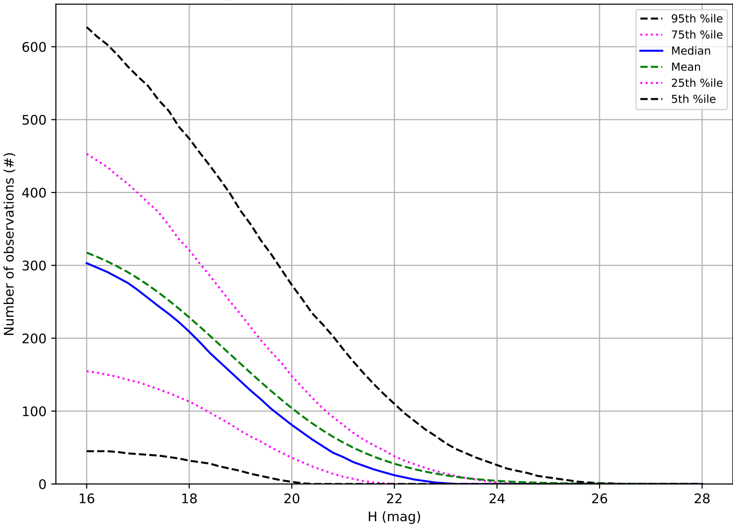
weather_cloudso4v3.4_10yrs: Number of observations PHA
