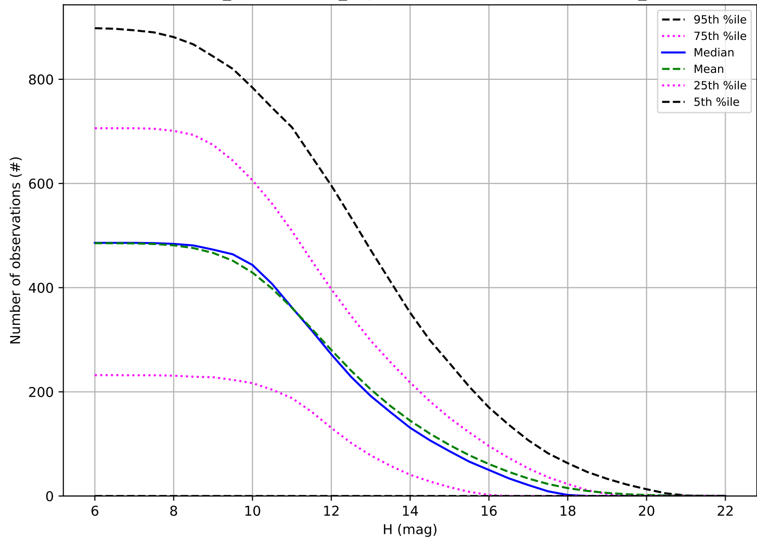
weather_cloudso4v3.4_10yrs: Number of observations OCC_r5
