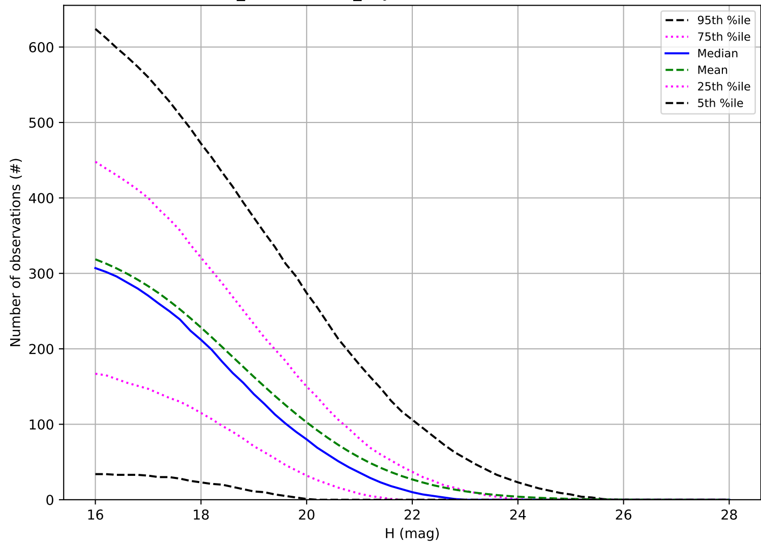
weather_cloudso4v3.4_10yrs: Number of observations NEO
