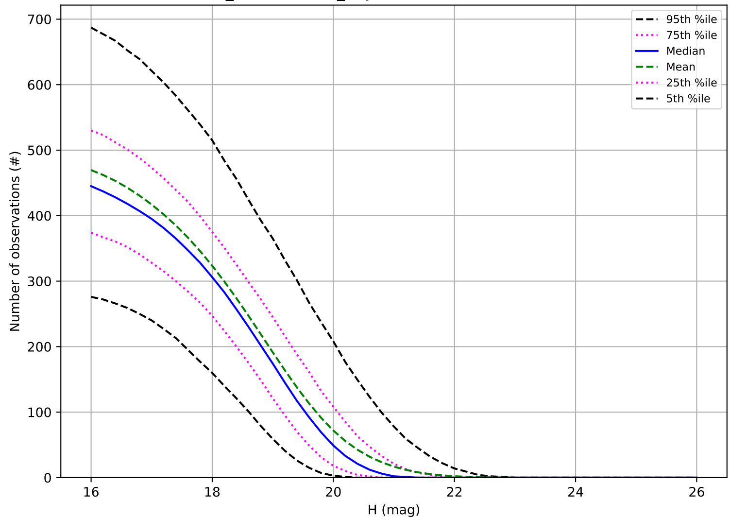
weather_cloudso4v3.4_10yrs: Number of observations MBA
