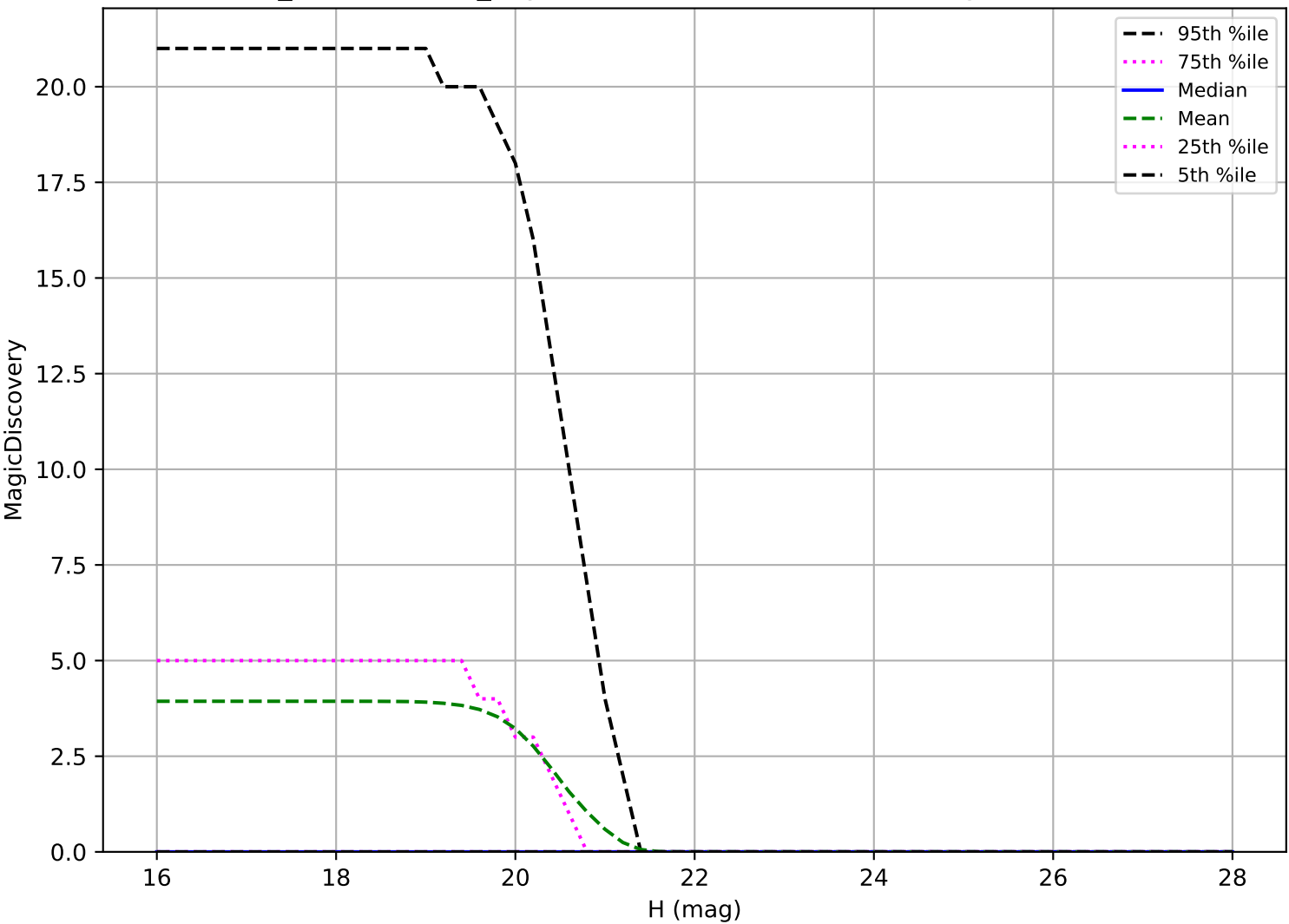
weather_cloudso4v3.4_10yrs: Vatira 6 detections in 60 nights detection loss
