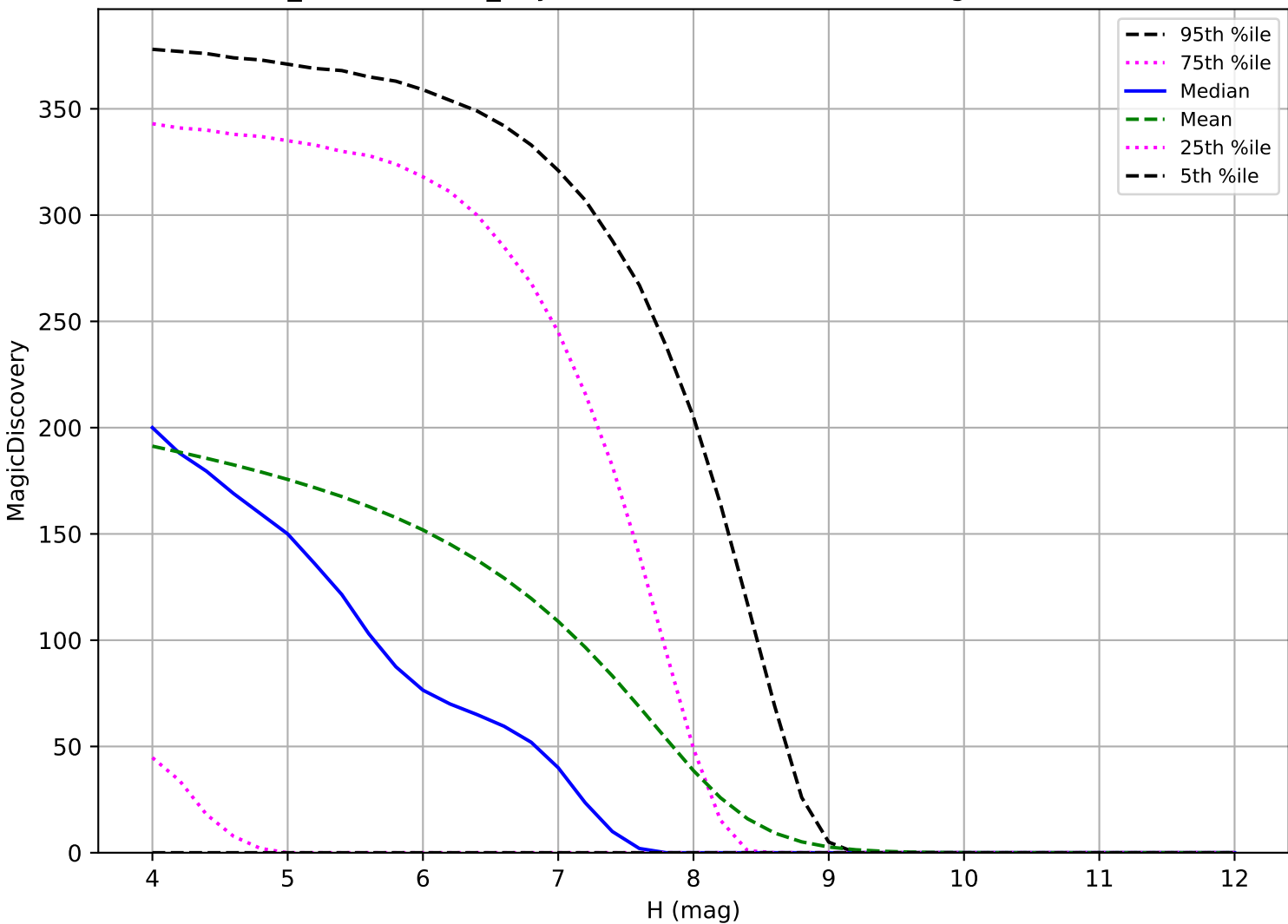
weather_cloudso4v3.4_10yrs: TNO 6 detections in 60 nights detection loss
