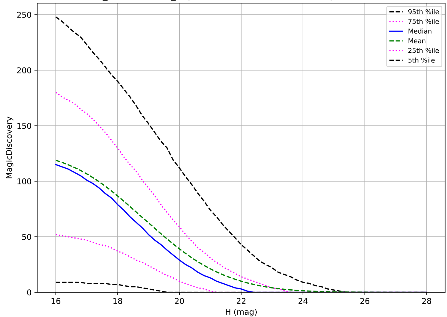
weather_cloudso4v3.4_10yrs: PHA 6 detections in 60 nights detection loss
