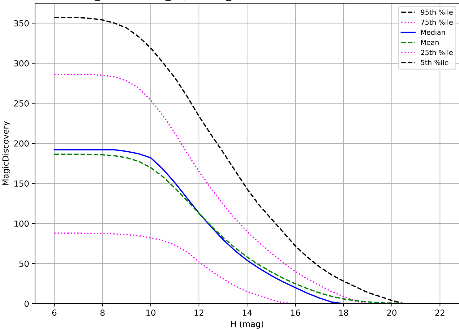
weather_cloudso4v3.4_10yrs: OCC_r5 6 detections in 60 nights detection loss
