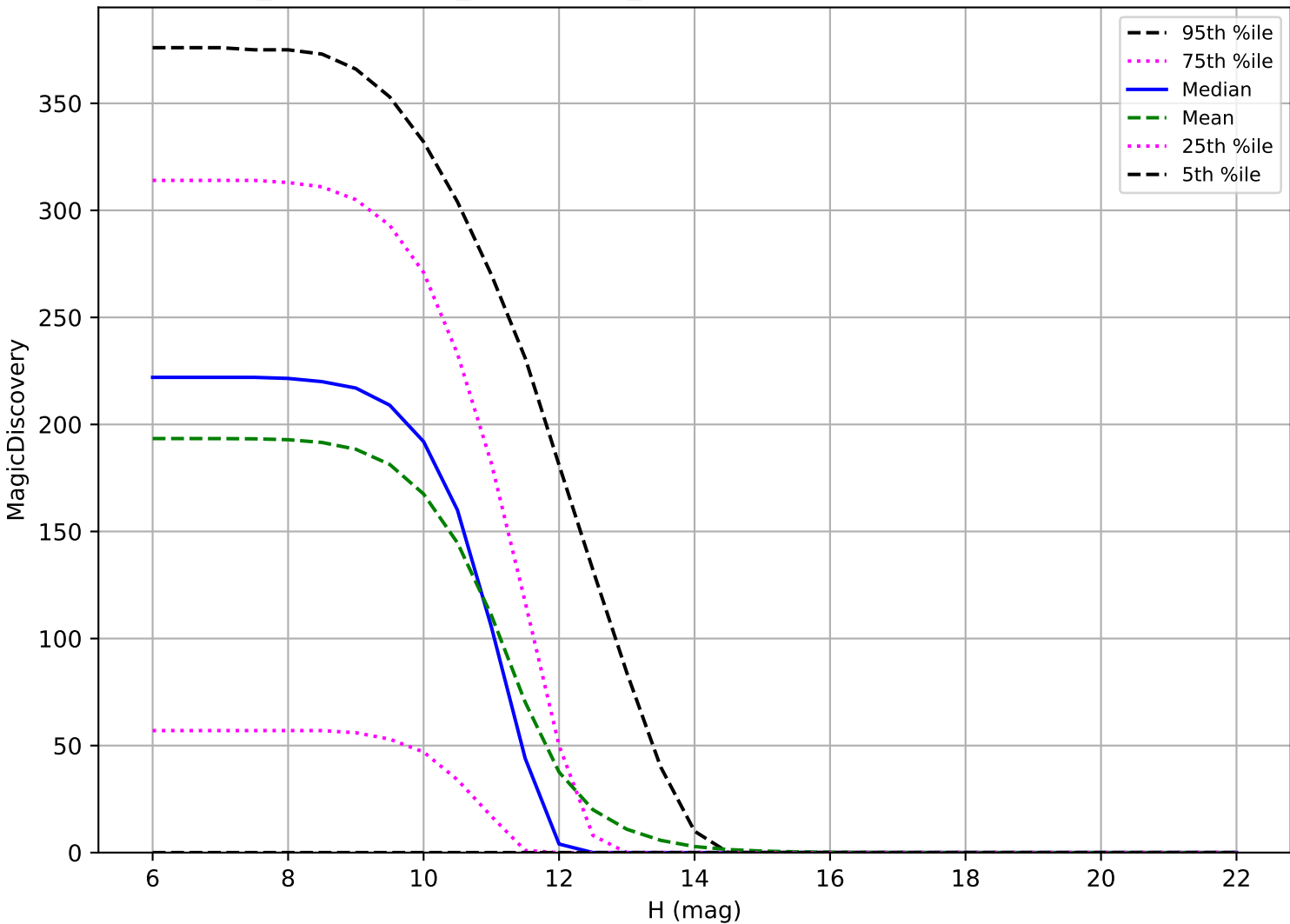
weather_cloudso4v3.4_10yrs: OCC_r20 6 detections in 60 nights detection loss
