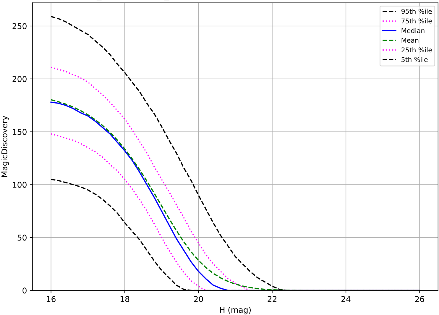
weather_cloudso4v3.4_10yrs: MBA 6 detections in 60 nights detection loss
